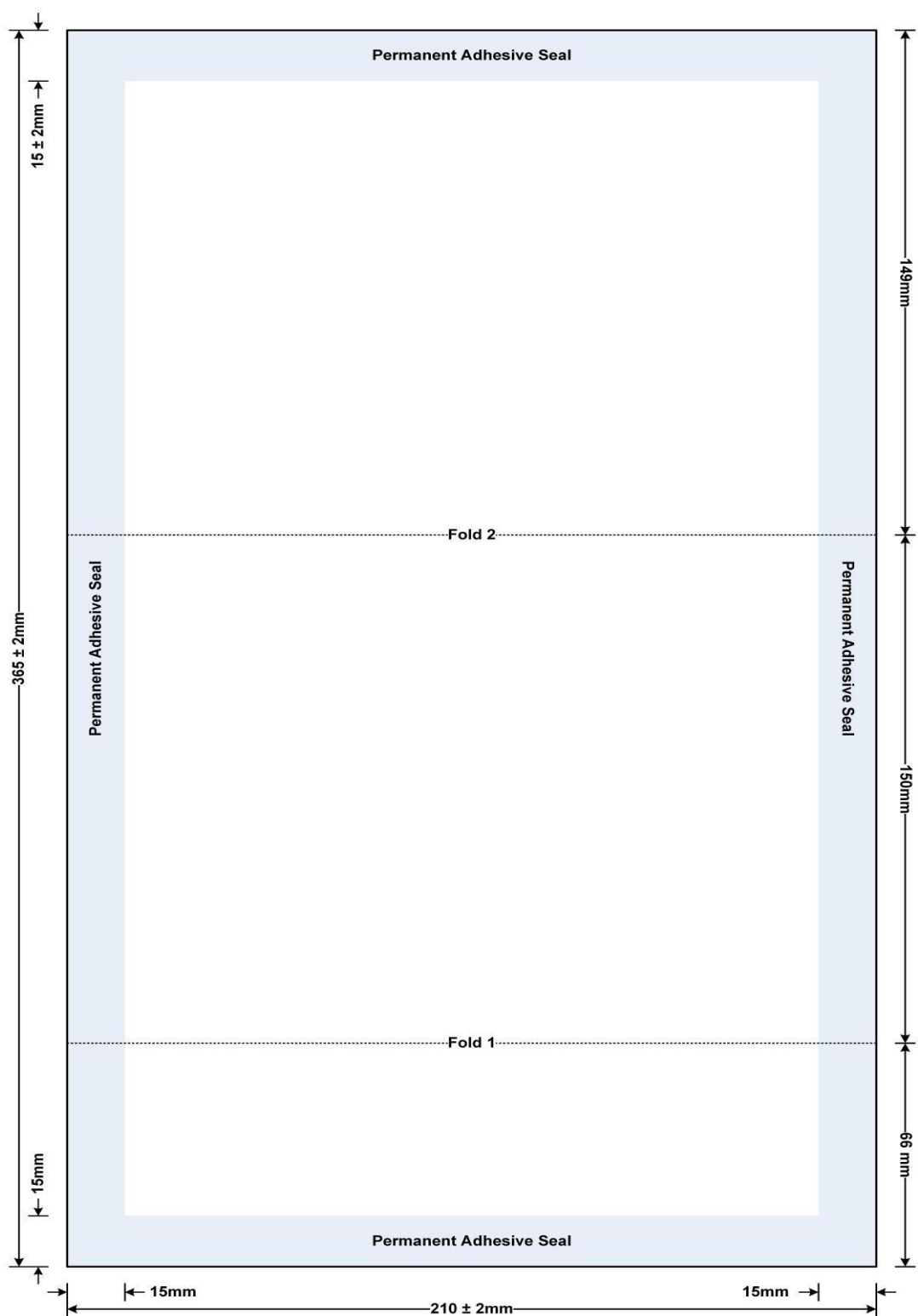
Figure 43: Physical Construction
