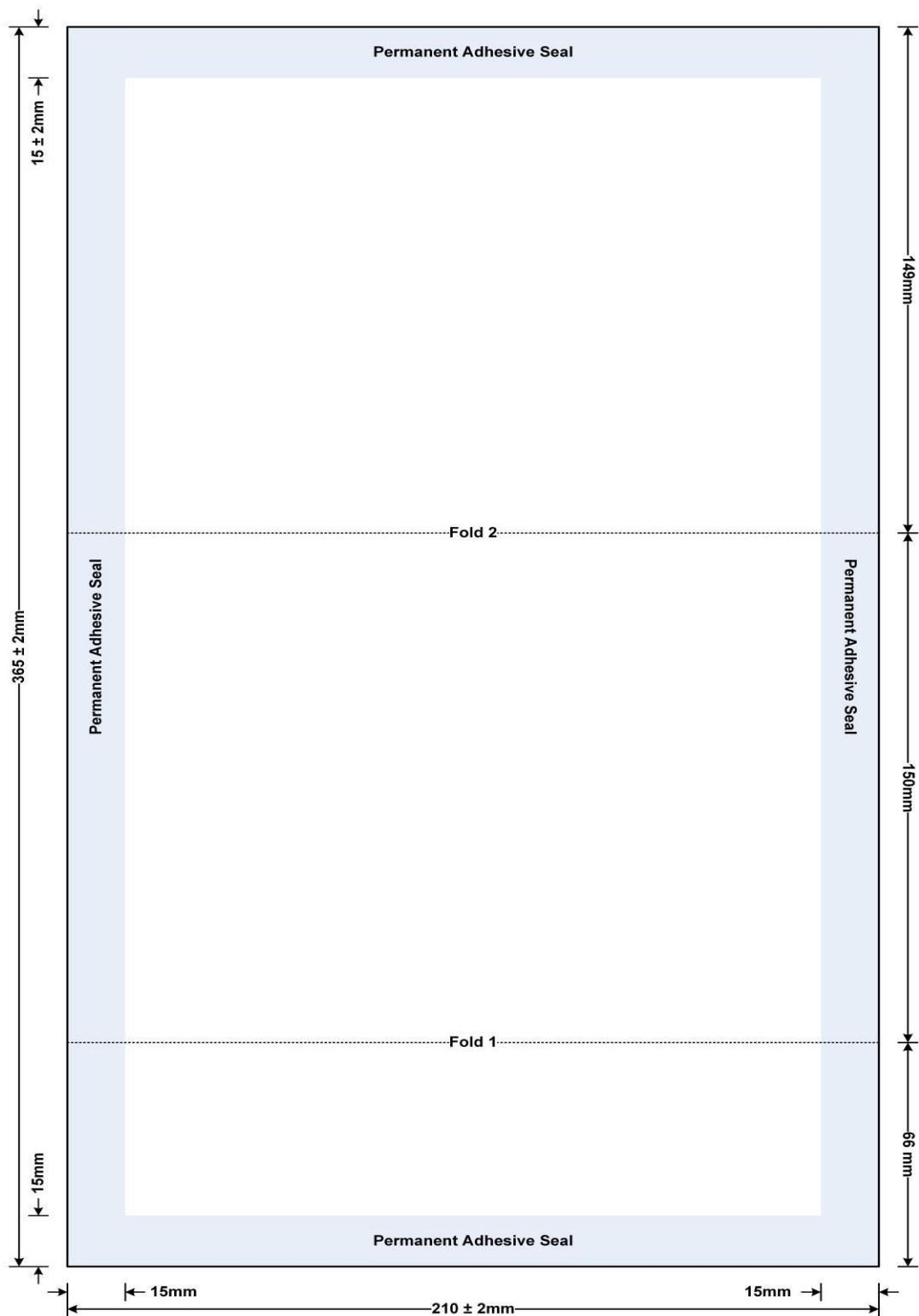
Figure 43: Physical Construction
